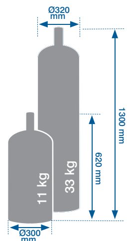
Propane gas cylinder
