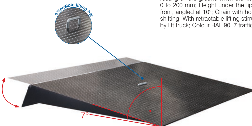
Ramp with movable lip
